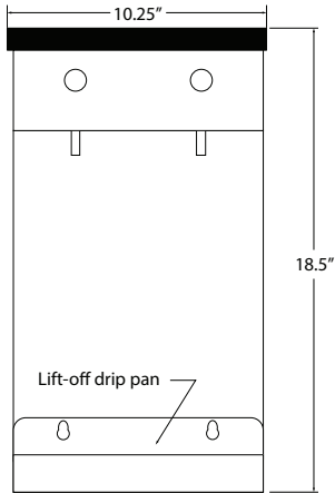
CM-2PB Front View
