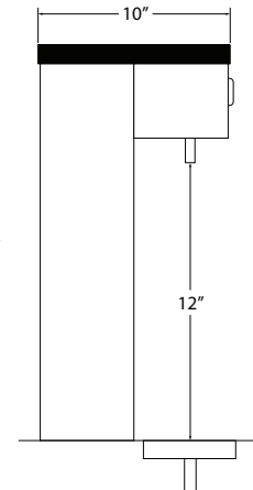
CM-2PB-RDP Side View
