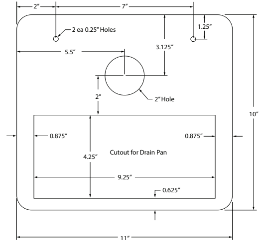
Recessed Drain Pan (RDP) Cutout Dimensions
