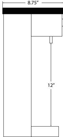
CM-2PB Side View
